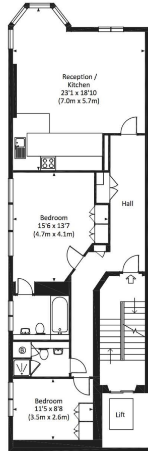
SECOND FLOOR
